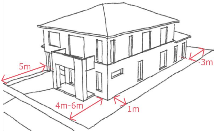
Diagram 3.3.1 Setbacks
