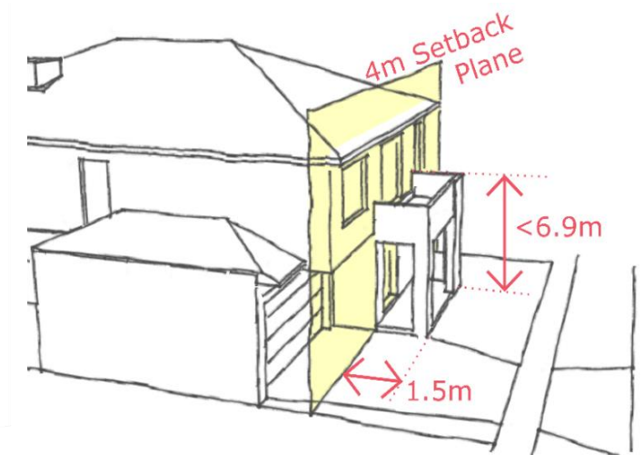
Diagram 3.3.2 Encroachments
